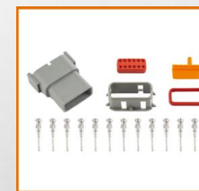
12-PIN CONNECTORS
